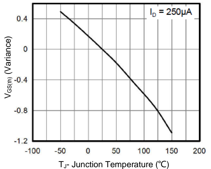
Figure 10. Threshold Voltage vs. Junction Temperature
