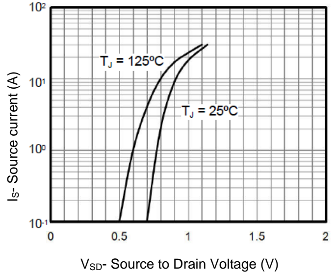
Figure 8. Body Diode Forward Voltage
