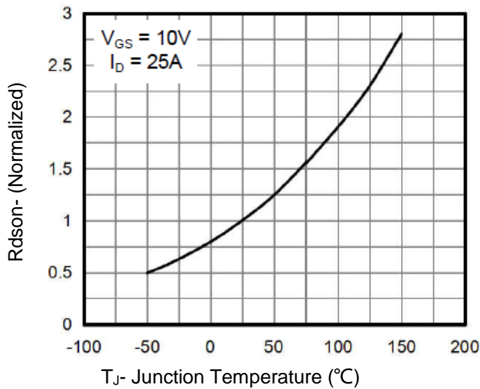
Figure 9. On- Resistance vs. Junction Temperature
