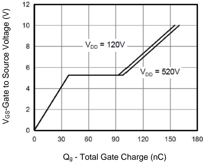
Figure 7. Gate Charge
