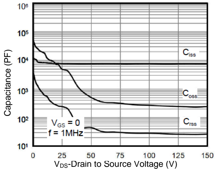
Figure 6. Capacitance
